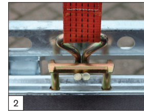
2 Standard: with TÜV certified load securing system with 1000 daN (Kg) for each fixing point.
