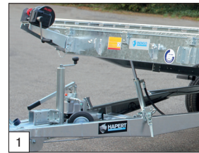
1 Standard: a double functioning tilting system, a 3,5t. coupling and a fixed Combi Protect Rail 80mm high.
