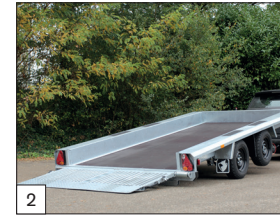
2 Standard: Indigo LT as a tiltable double axle, dimension 410 x 184 cm.
